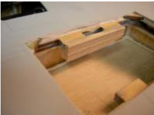
Modification to the forward ply mounting tabs for wing servos
