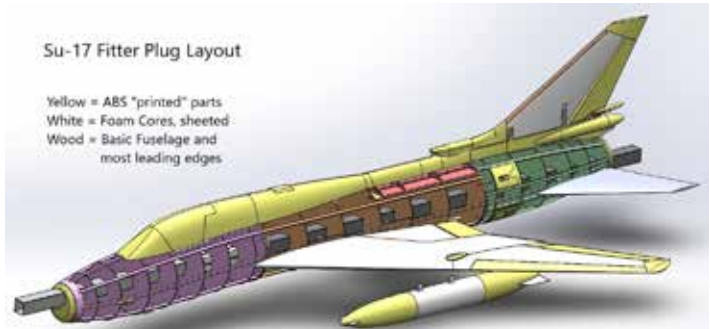
Screen shot of the Computer layout of plug.
