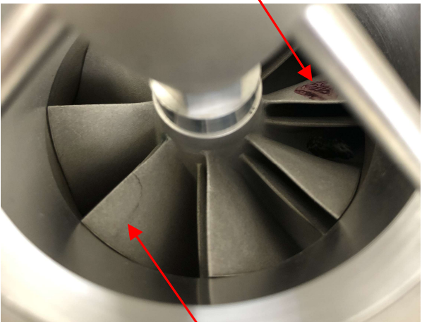
Hairline crack in compressor blade Apr 2022 (Rev 4)
